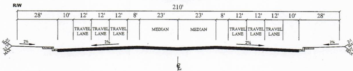
Figure 5.3: Typical Street Cross Sections in Imperial County
